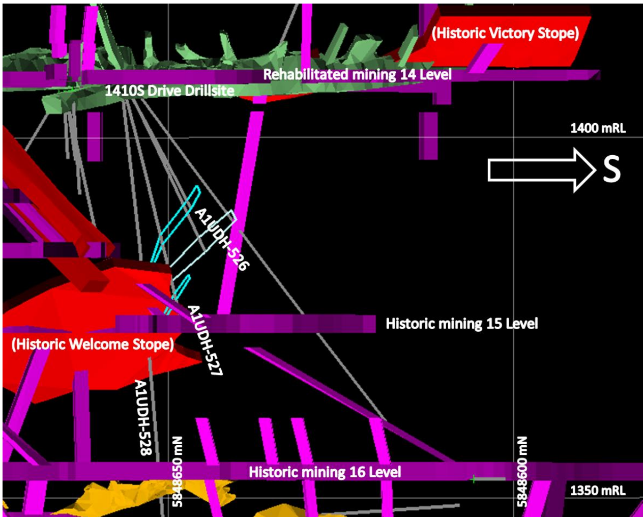
Figure 2: Longitudinal section looking East showing drilling traces (grey), modern drives (green) and the interpreted historic workings (magenta), surveyed historical (amber) and schematic interpretations of historical airleg stoping (red).
