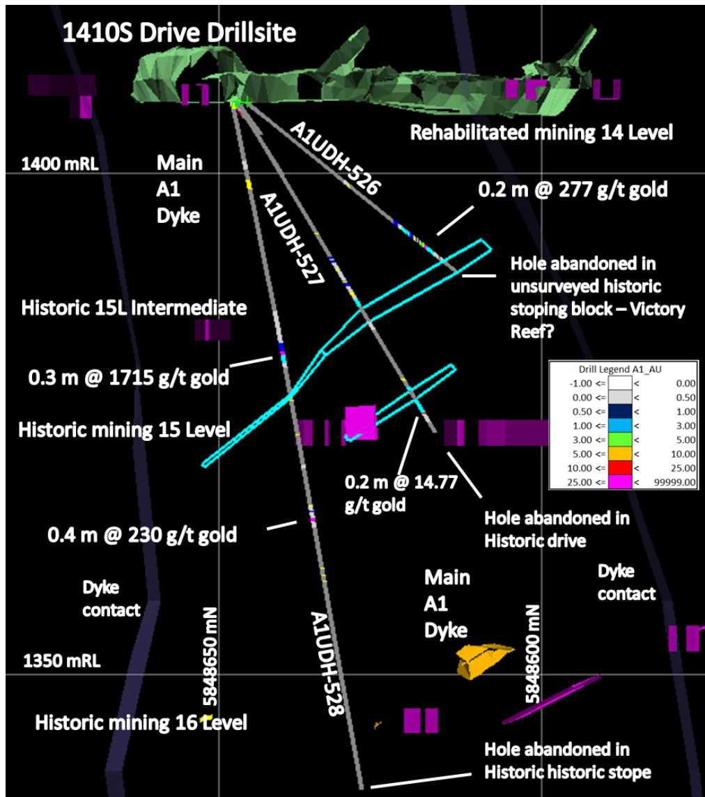
Figure 1: cross section viewed southeast along 230 Mine grid azimuth, illustrates the location of the drillholes A1UDH-526, -527 and -528 drilled from the 1410S Drive, with respect to the A1 Mine workings, reported in this announcement. Modern drives (green) and the interpreted historic workings (magenta), surveyed (amber) and unsurveyed historic stoping (blue).
